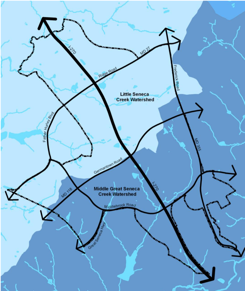
Figure 1: Watersheds
