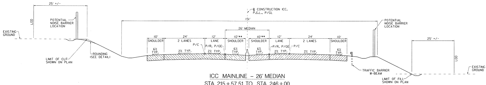
ICC MAINLINE - 26' MEDIAN AT WINTERS RUN STA. 215+57.51 TO STA. 246+00 (AREAS WITH RETAINING WALLS AND AREA WITH DECKOVER)
