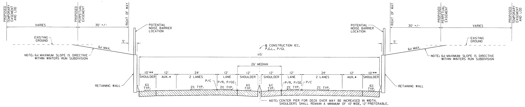
ICC MAINLINE - 26' MEDIAN AT WINTERS RUN STA. 215+57.51 TO STA. 246+00 (AREAS WITH RETAINING WALLS AND AREA WITH DECKOVER)
