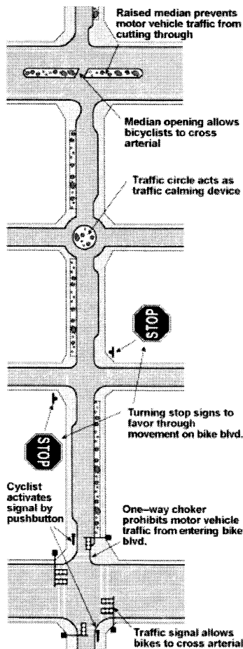
Figure C-1 Aerial view of a bicycle boulevard (Source: Oregon Department of Transportation)
