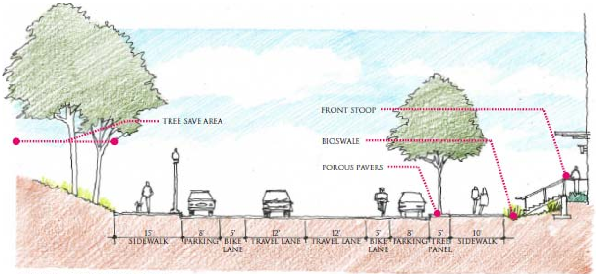
NEBEL STREET SECTION
