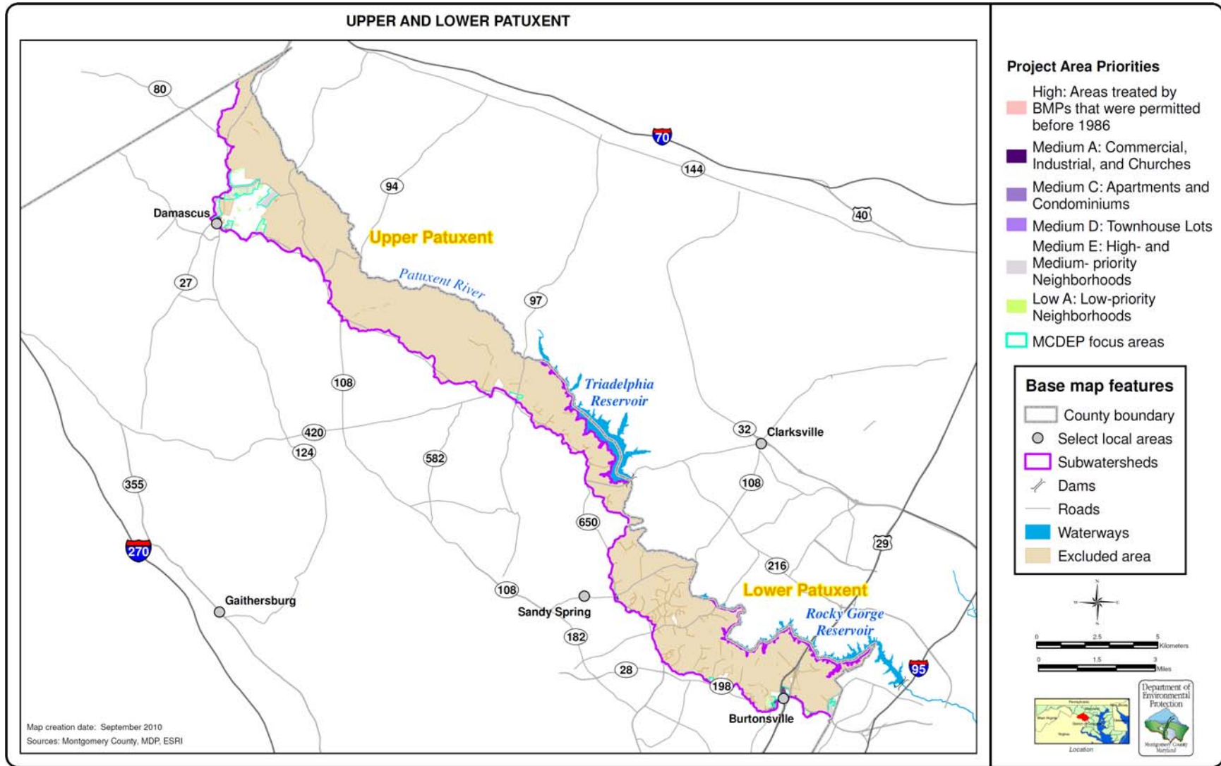
Figure 8: Project area priorities for candidate stormwater BMP retrofits in the Upper Patuxent and Lower Patuxent subwatersheds, Montgomery County, Maryland
