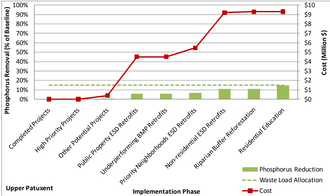
Figure 14: Cumulative reduction in total phosphorus (TP) loading over restoration practices implementation for Upper Patuxent subwatershed (Triadelphia Reservoir).
