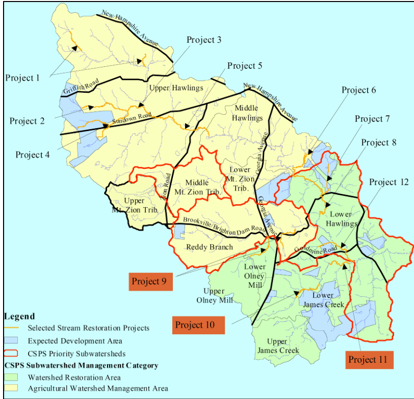
Figure 9: Twelve candidate stream bank stabilization and buffer enhancement projects in the Hawlings River subwatershed. Top 3 ranked projects are highlighted in orange. (Charles P. Johnson and Associates and Environmental Quality Resources, LLC 2003)
