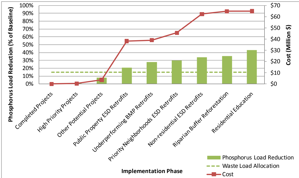
Figure 15: Cumulative reduction in TP loading over restoration practices implementation for Hawlings River and Lower Patuxent subwatersheds (Rocky Gorge Reservoir).
